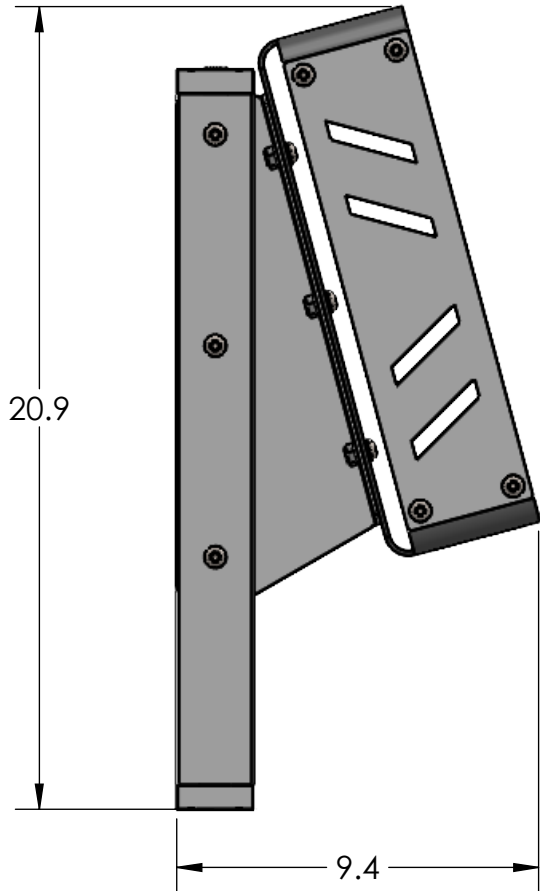
STORAGE POSITION
