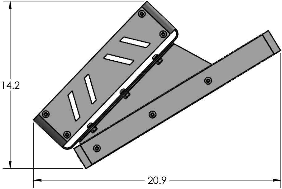
DOWN POSITION
