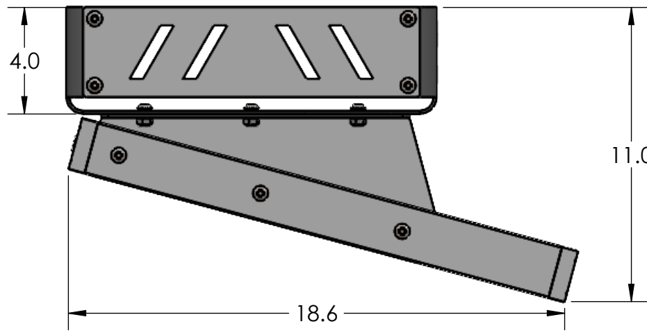
RIDE POSITION
