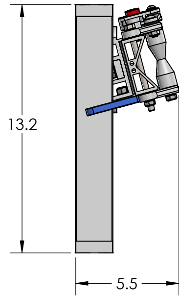
STORAGE POSITION
