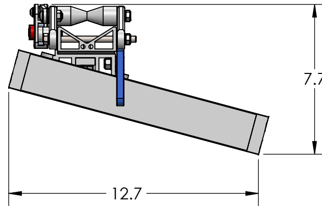
RIDE POSITION
