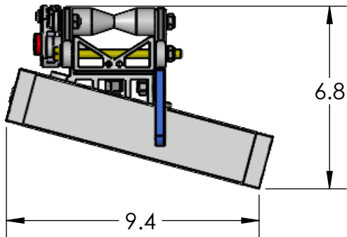
RIDE POSITION
