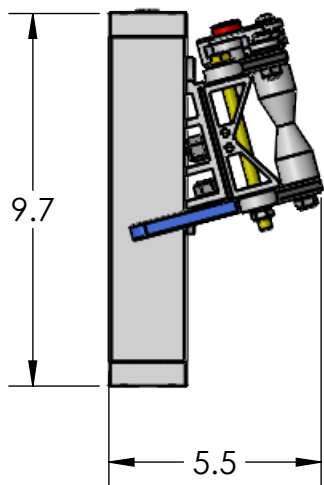
STORAGE POSITION
