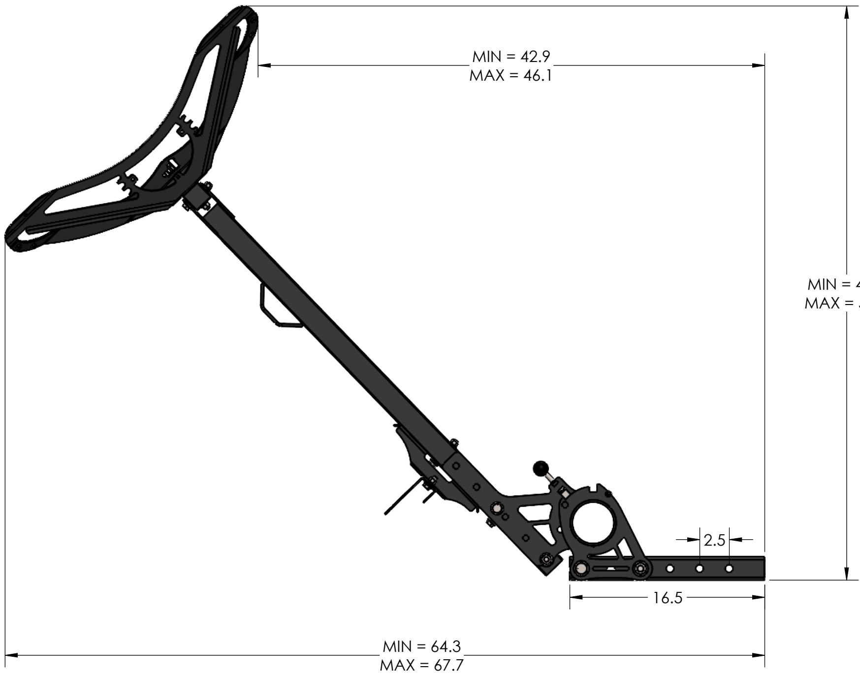
DOWN POSITION
