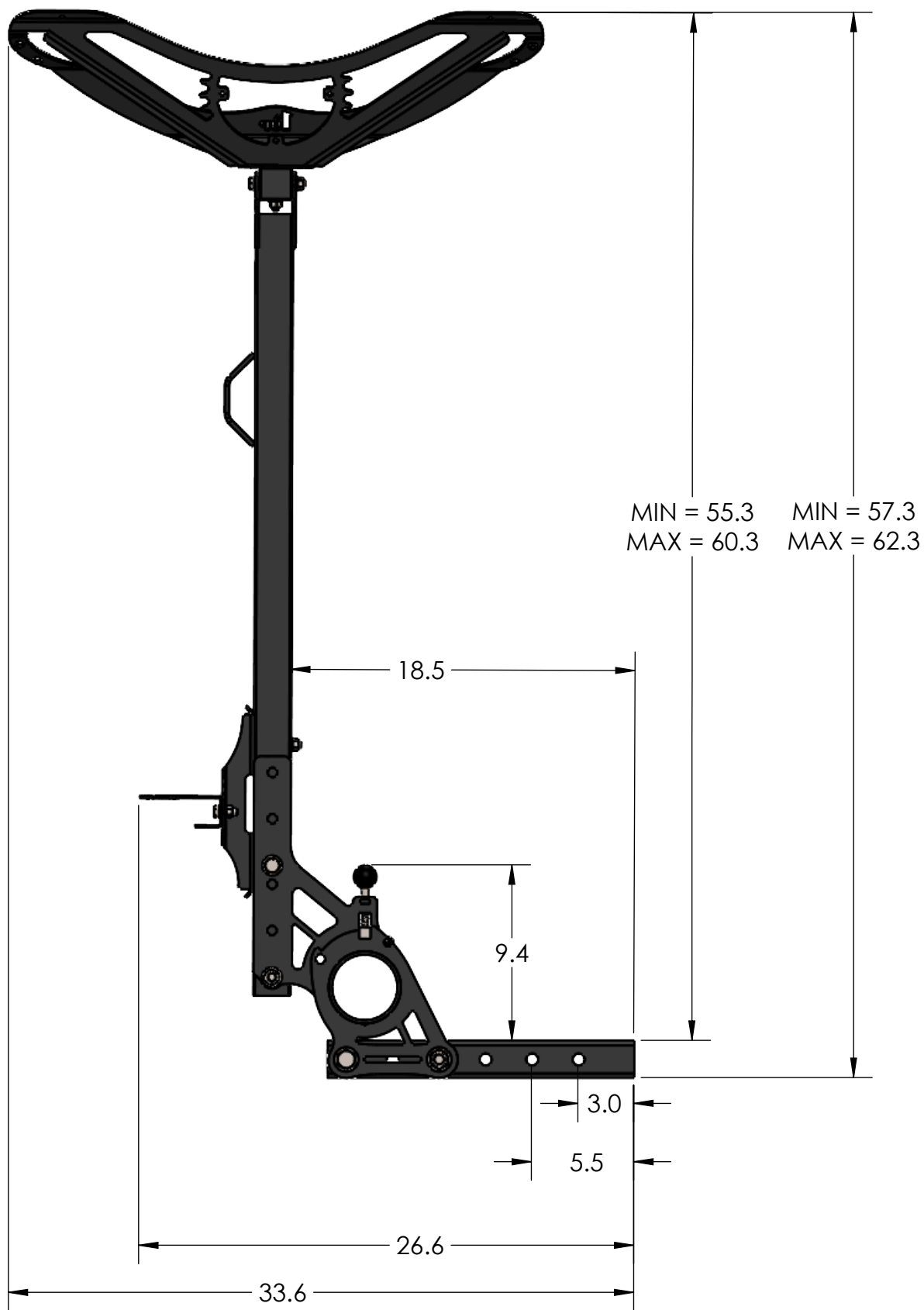
RIDE POSITION
