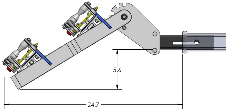
BASE RACK W/ ONE ADD-ON
