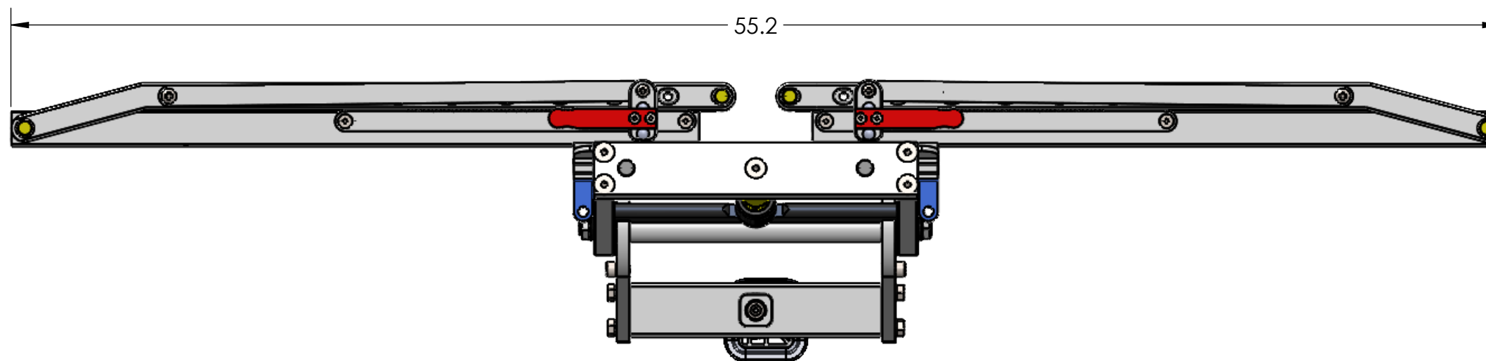
OVERALL WIDTH
