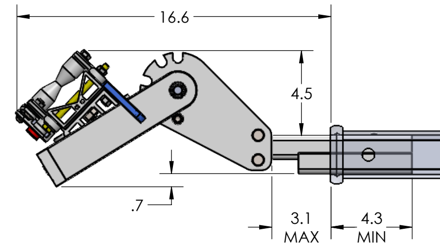
DOWN POSITION
